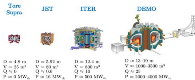
Figure 35 Size of ITER and DEMO reactors
